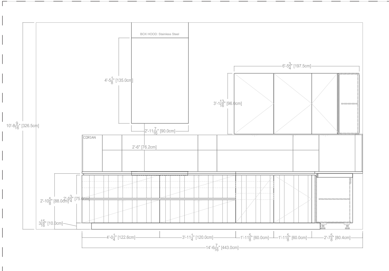
ARTEX KITCHEN - ELEVATION A
