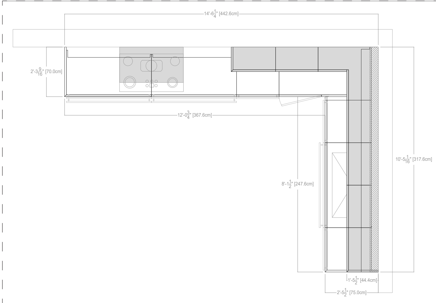
ARTEX KITCHEN - PLAN VIEW
