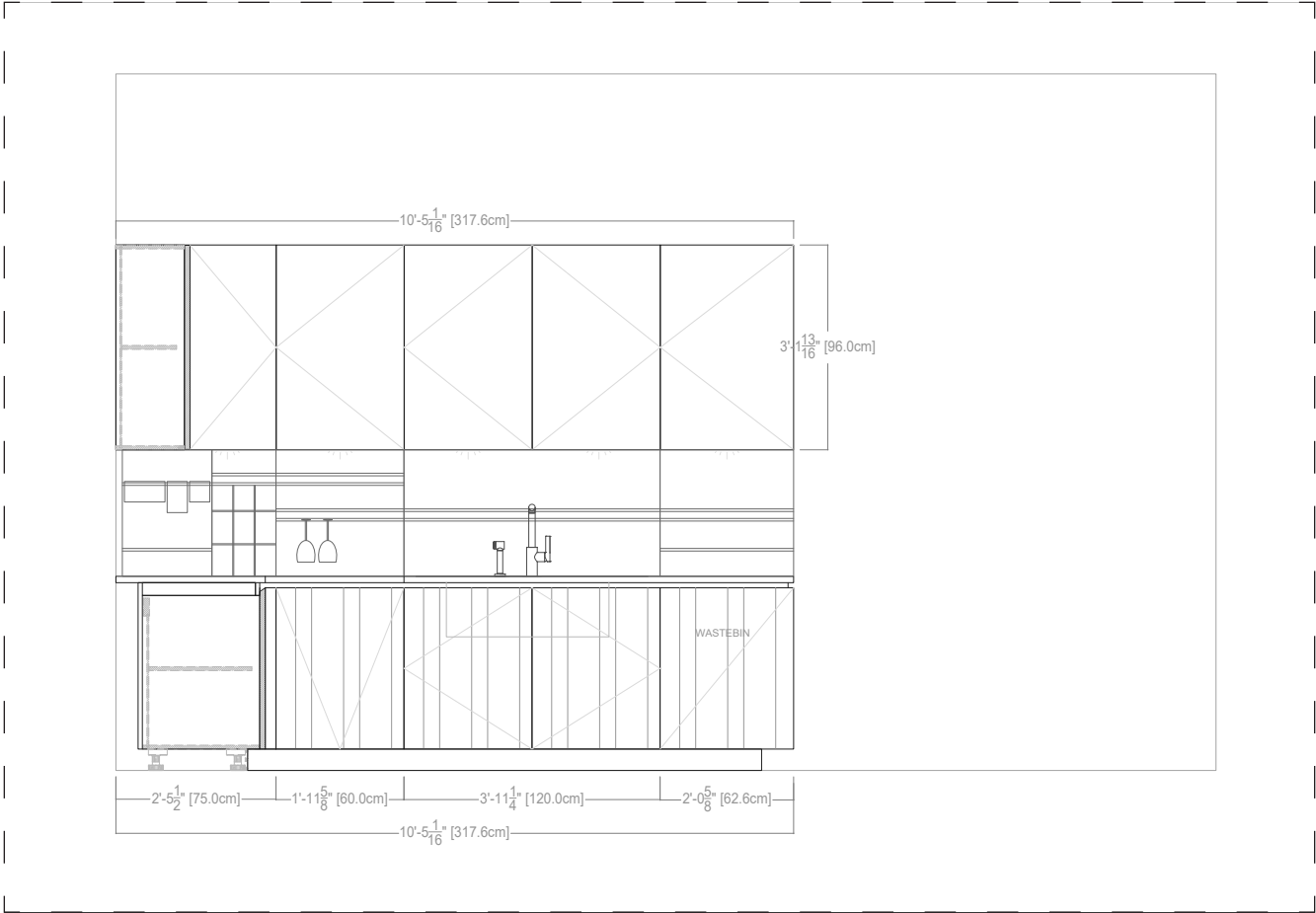
ARTEX KITCHEN - ELEVATION B
